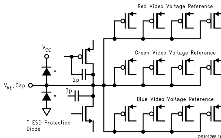
FIGURE 13. Pin 3 ( V_{\text{REF}} \text{ Cap} )
