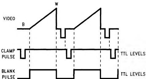
FIGURE 7. Timing Diagram
