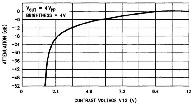
Attenuation vs Contrast Voltage
