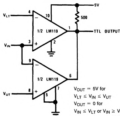
Window Detector
