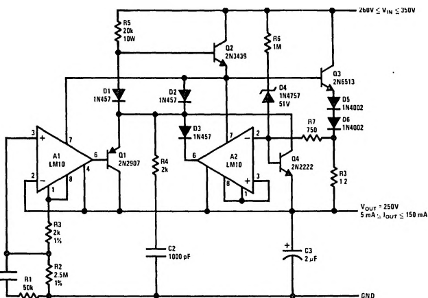
Protected HV Regulator
