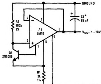
Negative Regulator
