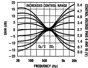
FIGURE 2: Tone Characteristic (Gain vs Frequency)
