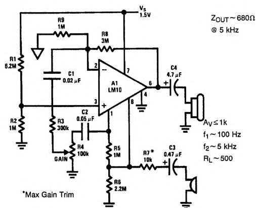
Microphone Amplifier
