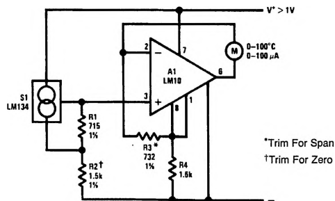
Thermometer
