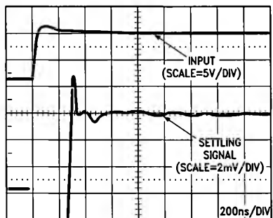
Settling Signal
