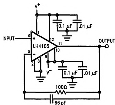
FIGURE 4. Unity Gain Follower
