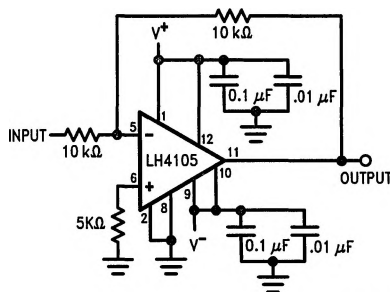
FIGURE 6. Unity Gain Inverter
