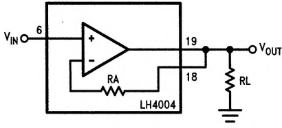
FIGURE 5. Unity Gain Buffer
