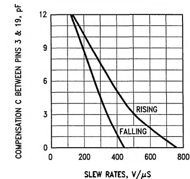
FIGURE 4. Slew Rates vs Compensation C
