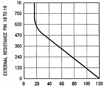
BANDWIDTH IN MHz FOR UNITY GAIN CONFIGURATION
