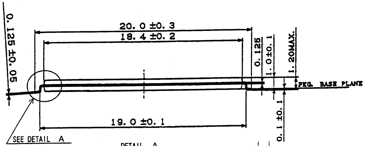
DETAIL A
