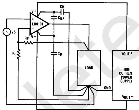
FIGURE 1. Single-Point Grounding
