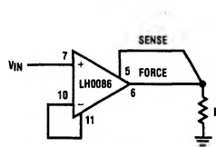
FIGURE 4. Remote Output Sense
