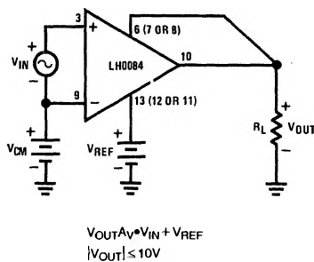
FIGURE 12. Output Offset Connection
