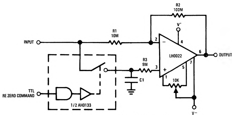
Re-Zeroing Amplifier
