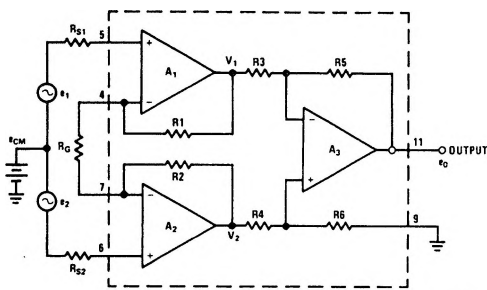
FIGURE 1. Simplified LH0036
