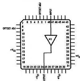
Leadless Chip Carrier
