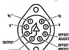
LH0063K Metal Can Package
