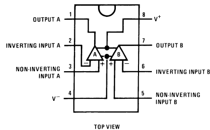
Figure 1. Dual-In-Line Package
