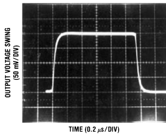
Figure 4. Small Signal Non-Inverting
