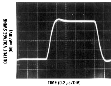
Figure 4. Small Signal Non-Inverting
