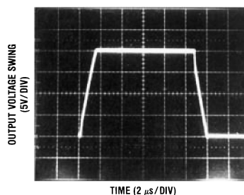
Figure 7. Current Limit ( R_L=100\Omega )
