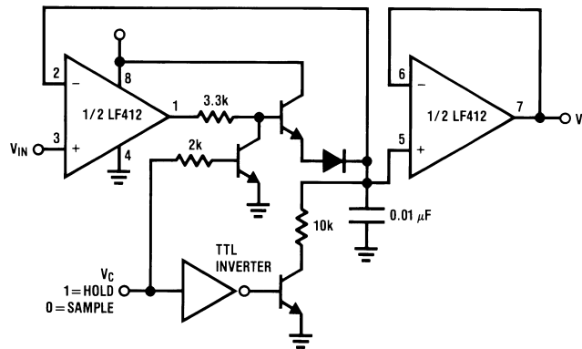
Figure 8. Single Supply Sample and Hold
