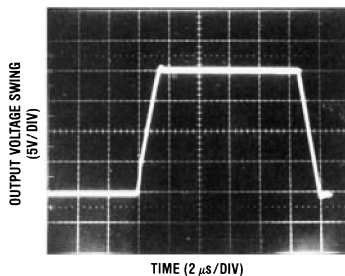
Figure 6. Large Signal Non-Inverting
