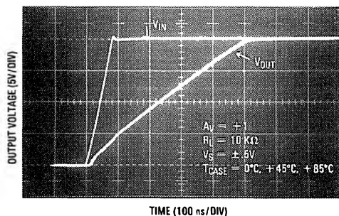
Step Response
