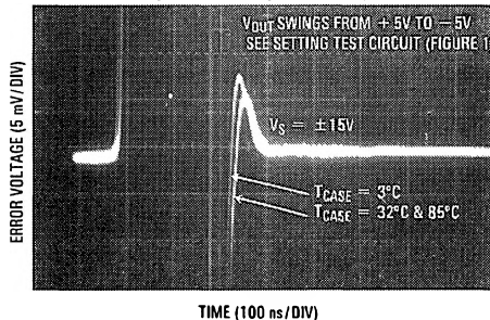
Settling Time—Negative Output Swing
