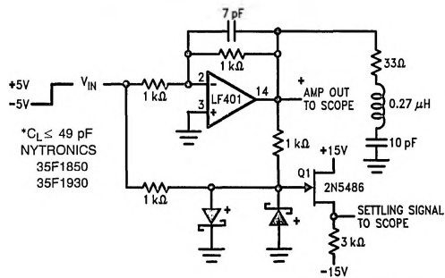
FIGURE 1. Simplified Settling Time Test Circuit (See Text)
