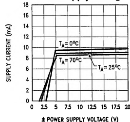
Power Supply Current vs. Power Supply Voltage
