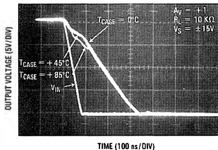
Step Response
