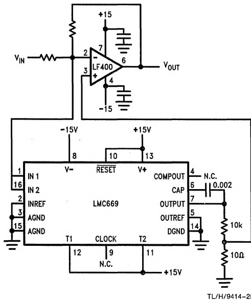
FIGURE 4b. Automatic Offset Adjustment Using LMC669
