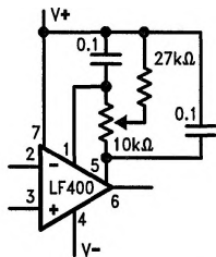
FIGURE 4a. V_{0s} Adjust Circuit
