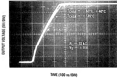
Step Response
