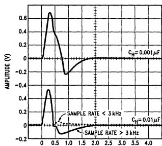
Output Transient at Start of Sample Mode
