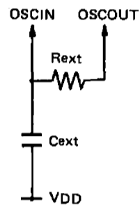
Fig. 12 RC oscillation
