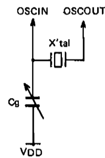
Fig. 7 Crystal oscillator
