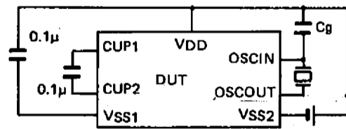
Fig. 5 Current dissipation, output voltage test circuit.
