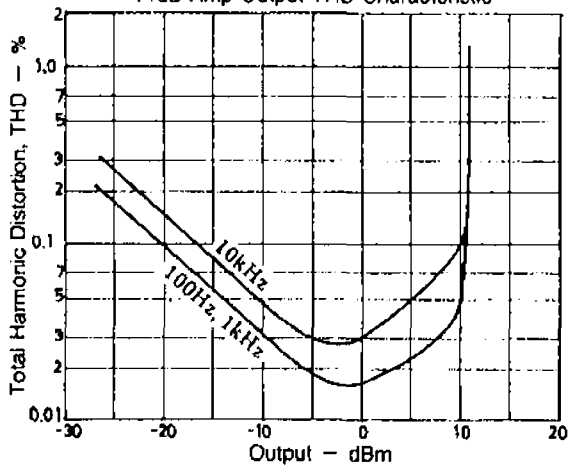
14dB Amp Output THD Characteristic
