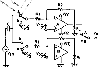
7 Channel separation CS
