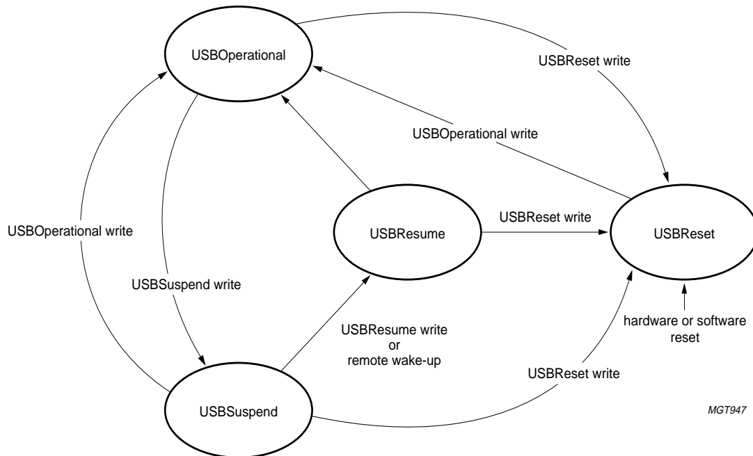
Fig 23. ISP1161A HC USB states.
