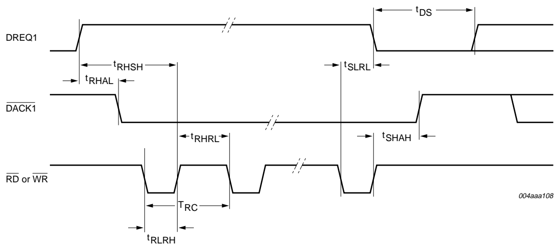
Fig 54. HC burst mode DMA timing.
