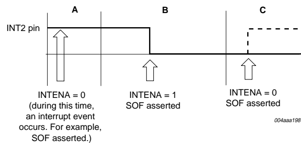
Fig 22. Behavior of bit INTENA bit.
