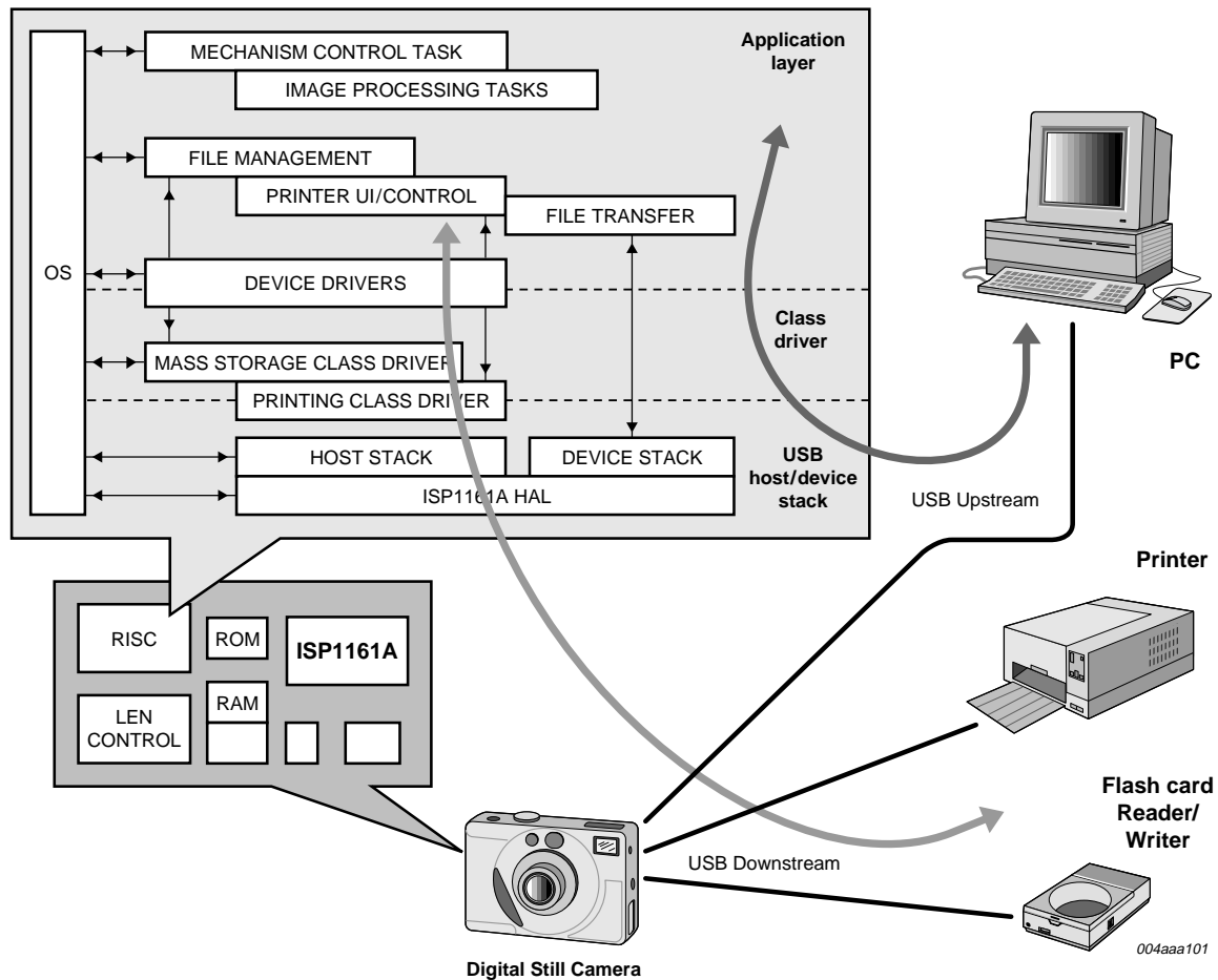
Fig 64. ISP1161A software model for DSC application.
