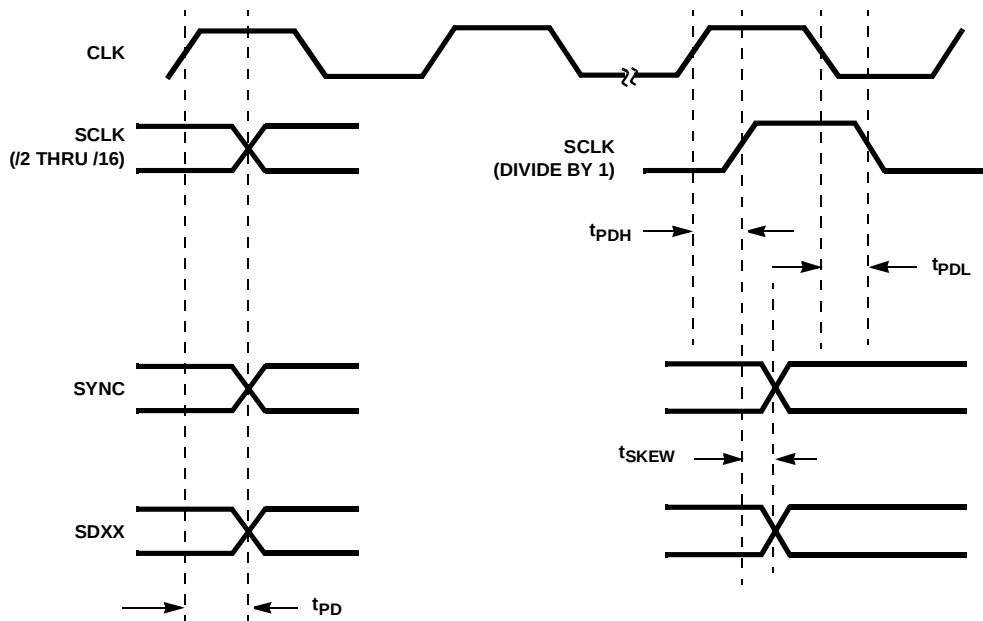
FIGURE 6. SERIAL OUTPUT TIMING
