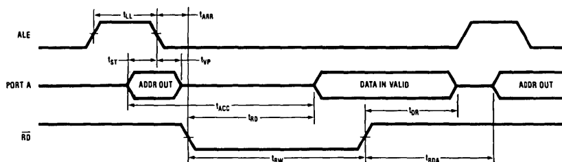
FIGURE 1. CPU and DMA Read Cycles
