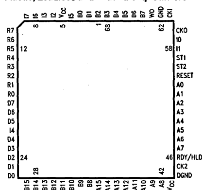
Plastic, Leadless and Leaded Chip Carriers
