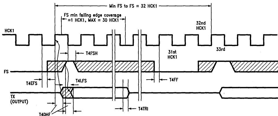
Serial Decoder Timing Diagrams (Mode 4)
