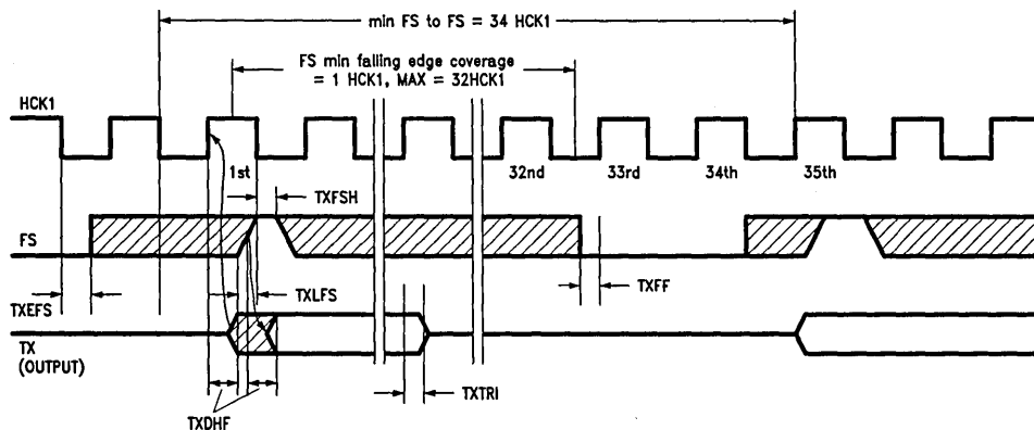
Serial Decoder Timing Diagrams (Mode 5,6,7)
