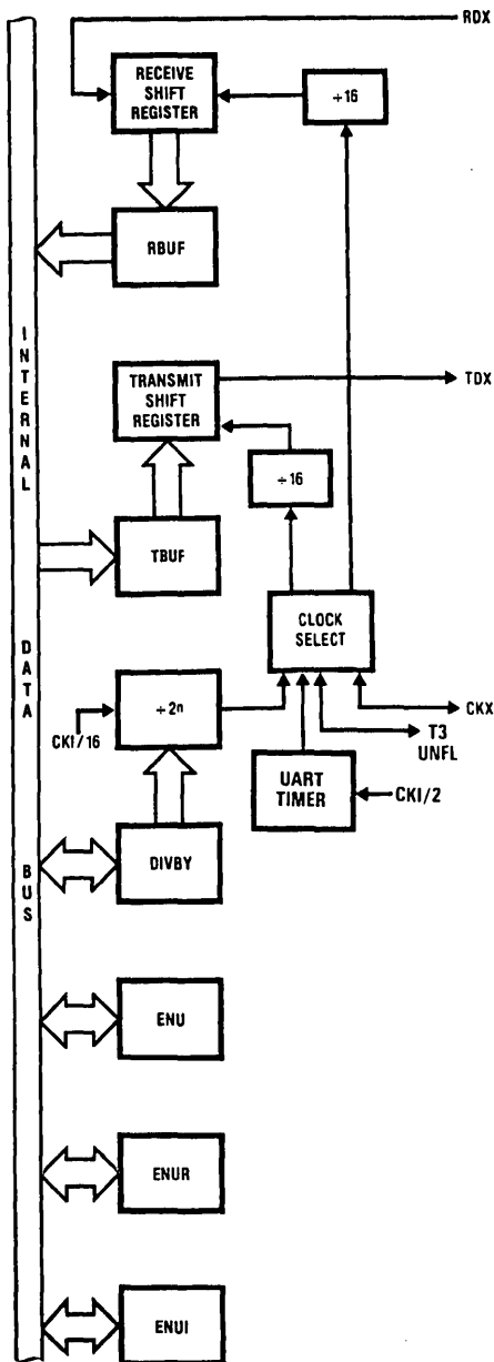
FIGURE 12. UART Block Diagram
