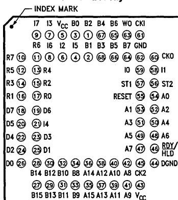
Pin Grid Array
