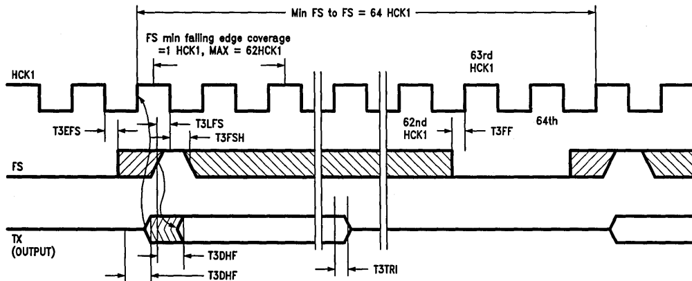
Serial Decoder Timing Diagrams (Mode 3)
