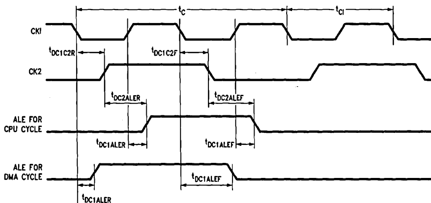
FIGURE 5. CK1, CK2 ALE Timing Diagram
