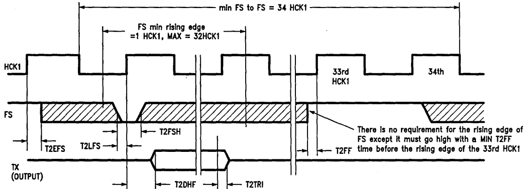
Serial Decoder Timing Diagrams (Mode 2)
