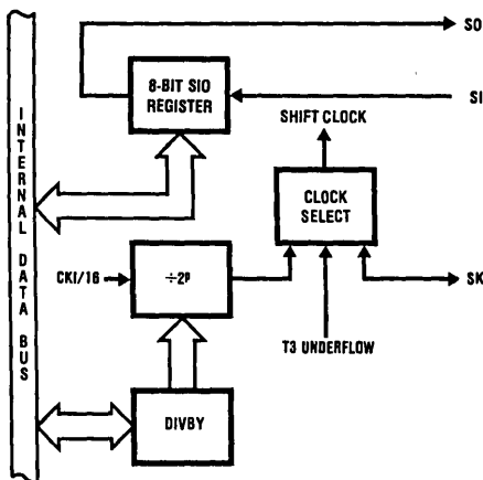
FIGURE 11. MICROWIRE/PLUS
