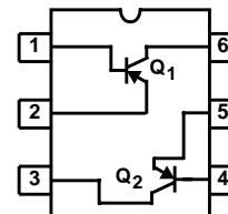
HFA3135 (SOT23) TOP VIEW
