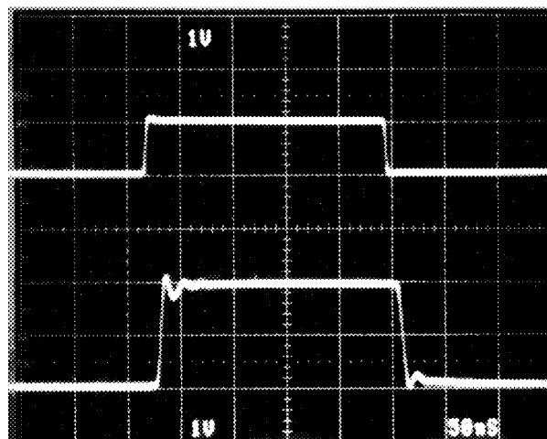
FIGURE 5. LARGE SIGNAL RESPONSE
