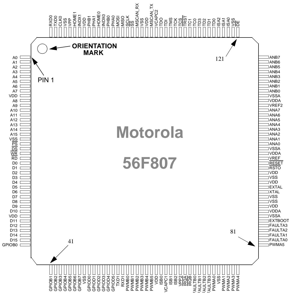
Figure 34. Top View, 56F807 160-pin LQFP Package
