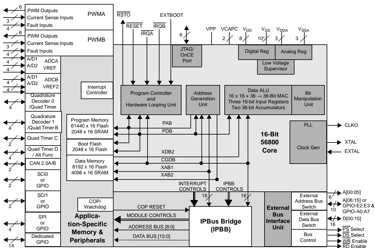
Figure 1. 56F807 Block Diagram
