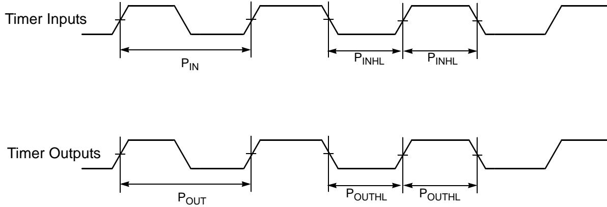
Figure 24. Timer Timing
