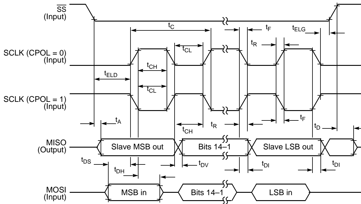
Figure 26. SPI Slave Timing (CPHA = 0)
