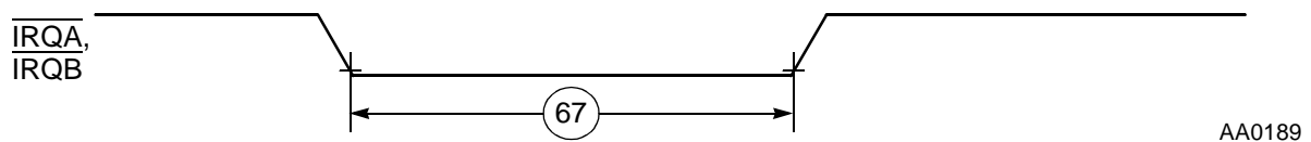
Figure 16. External Interrupt Timing (Negative-Edge-Sensitive)
