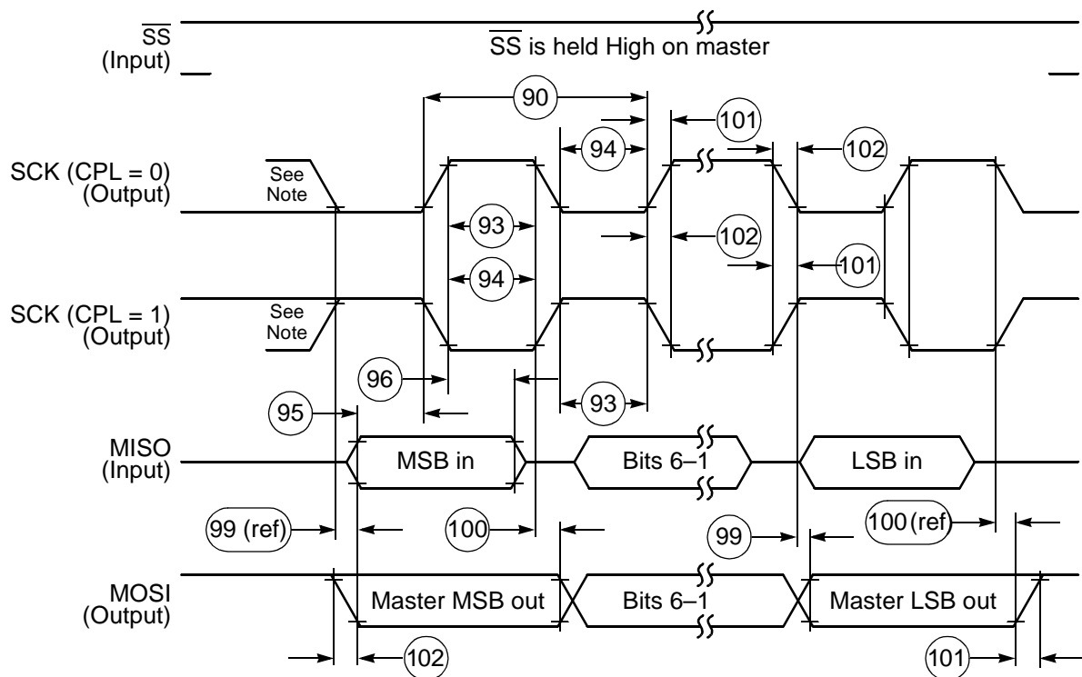
Figure 24. SPI Master Timing (CPH = 0)
