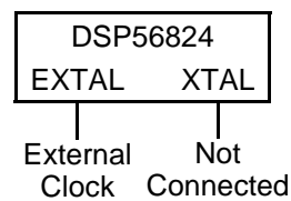
Figure 7. Connecting an External Clock Signal
