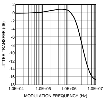
Figure 22. Typical Serializer Jitter Transfer Function at 43 MHz
