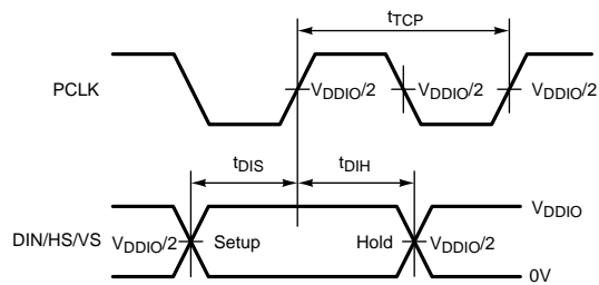
Figure 14. Serializer Setup/Hold Times
