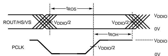
Figure 20. Deserializer Output Setup/Hold Times
