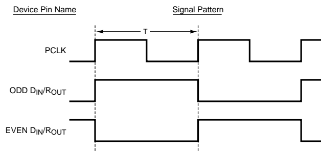
Figure 7. "Worst Case" Test Pattern
