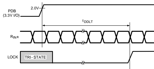
Figure 17. Deserializer Data Lock Time
