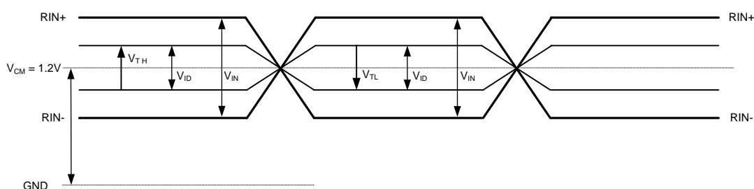
Figure 12. Differential VTH/VTL Definition Diagram
