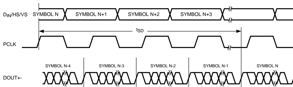
Figure 16. Serializer Delay
