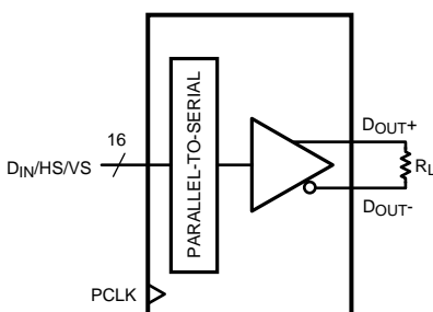
Figure 10. Serializer VOD DC Diagram
