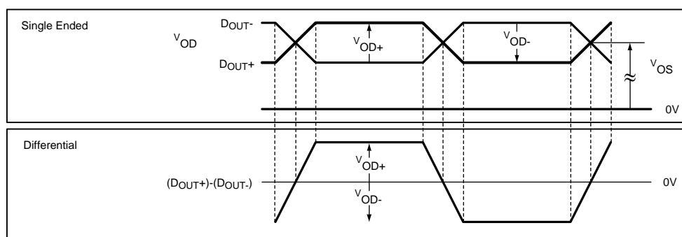
Figure 11. Serializer VOD DC Diagram
