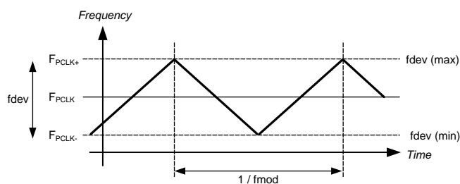
Figure 21. Spread Spectrum Clock Output Profile
