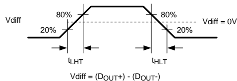
Figure 8. Serializer CML Output Load and Transition Times
