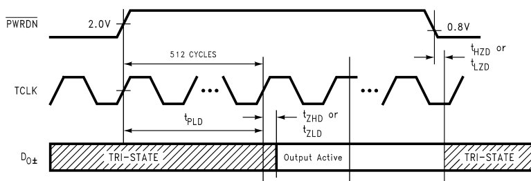
Figure 7. Serializer PLL Lock Time, and PWRDN TRI-STATE Delays
