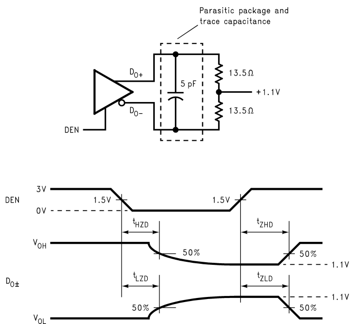
Figure 6. Serializer TRI-STATE Test Circuit and Timing
