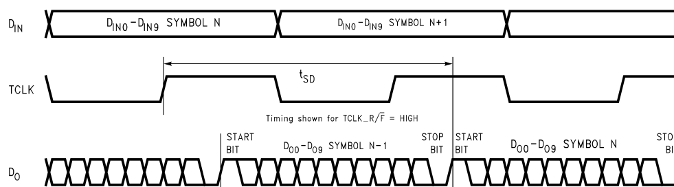
Figure 9. Serializer Delay
