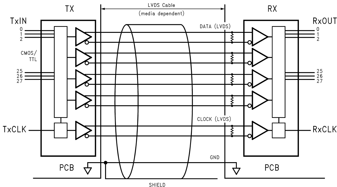
Figure 5. DS90CR288A
