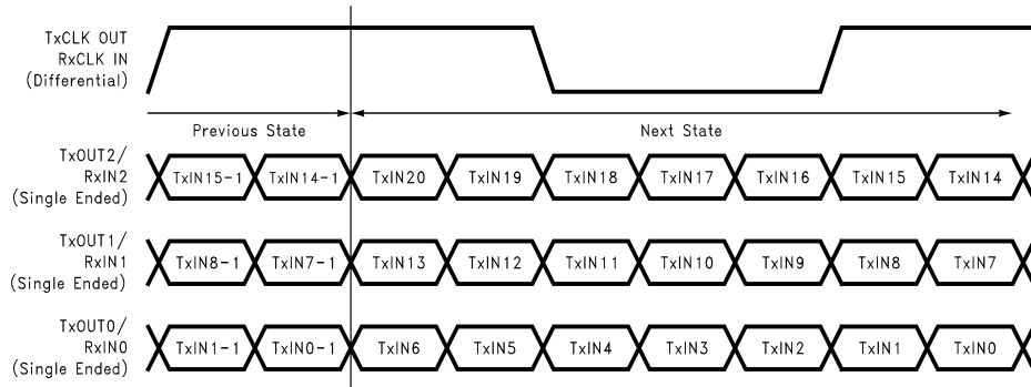
FIGURE 9. 21 Parallel TTL Data Inputs Mapped to LVDS Outputs
