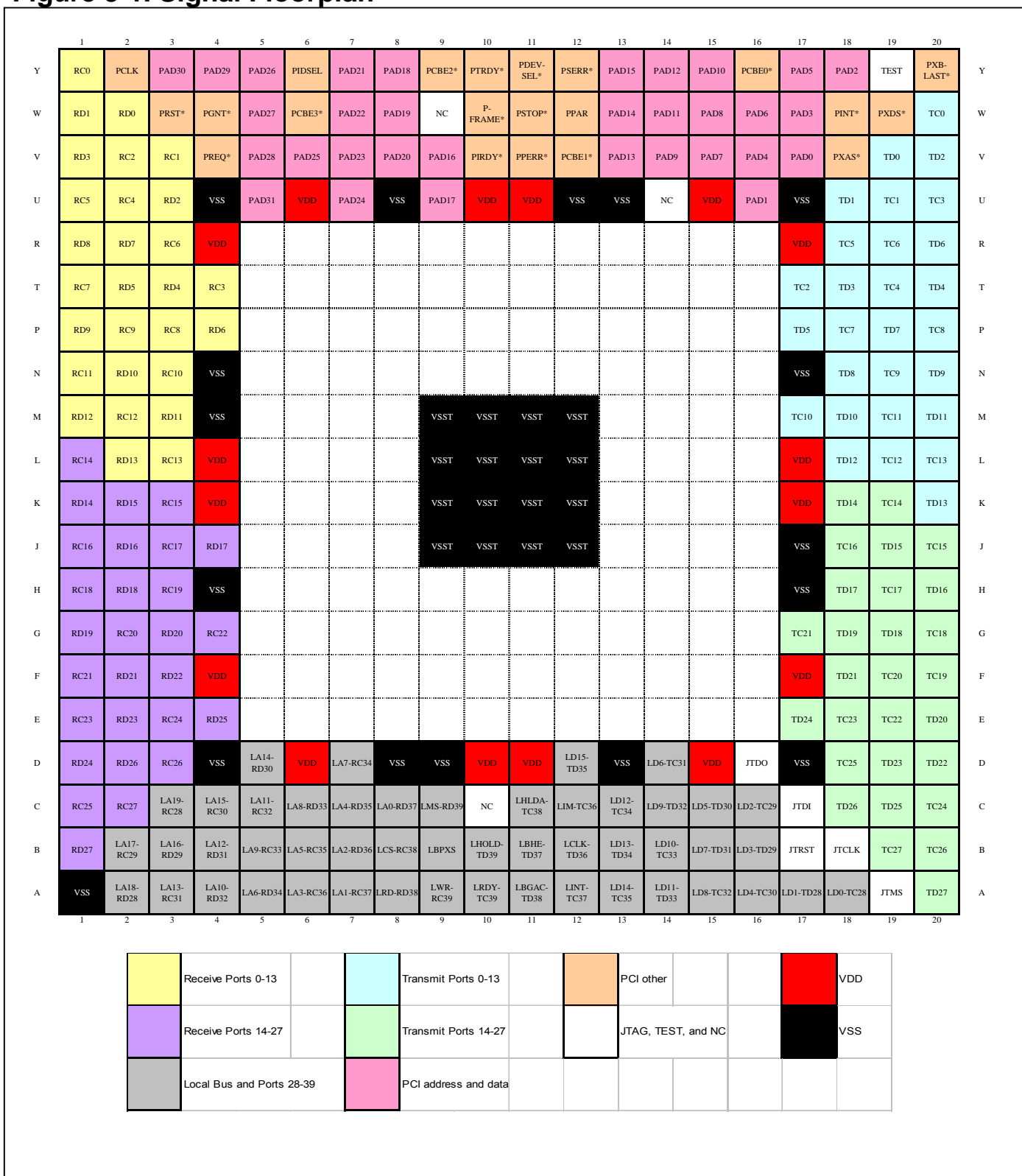
Figure 3-1. Signal Floorplan
