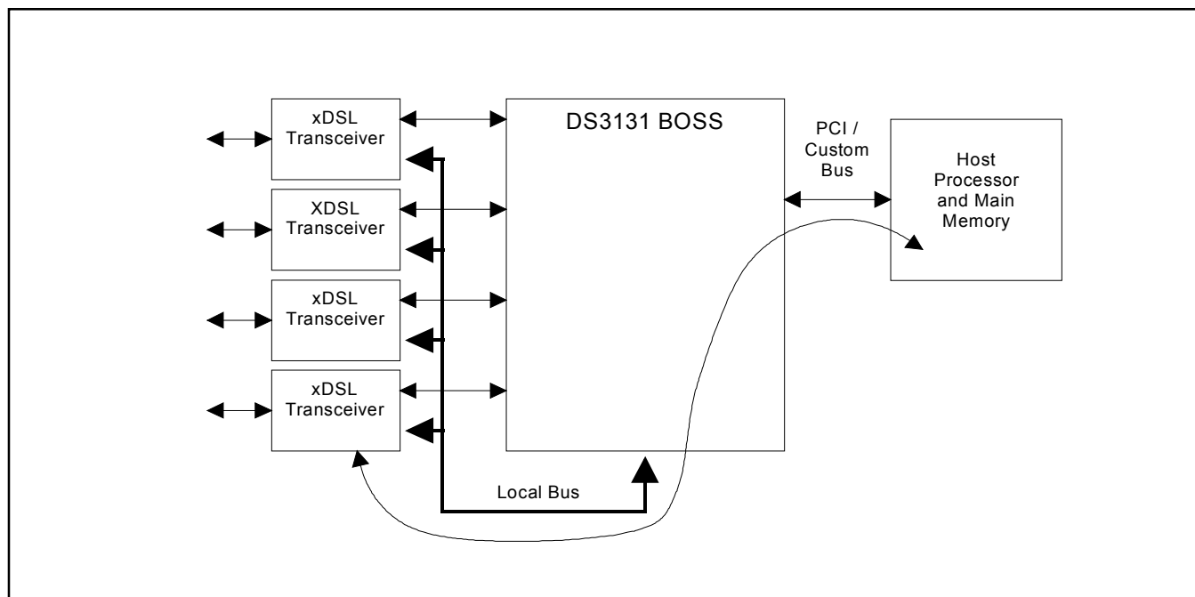
Figure 11-1. Bridge Mode
