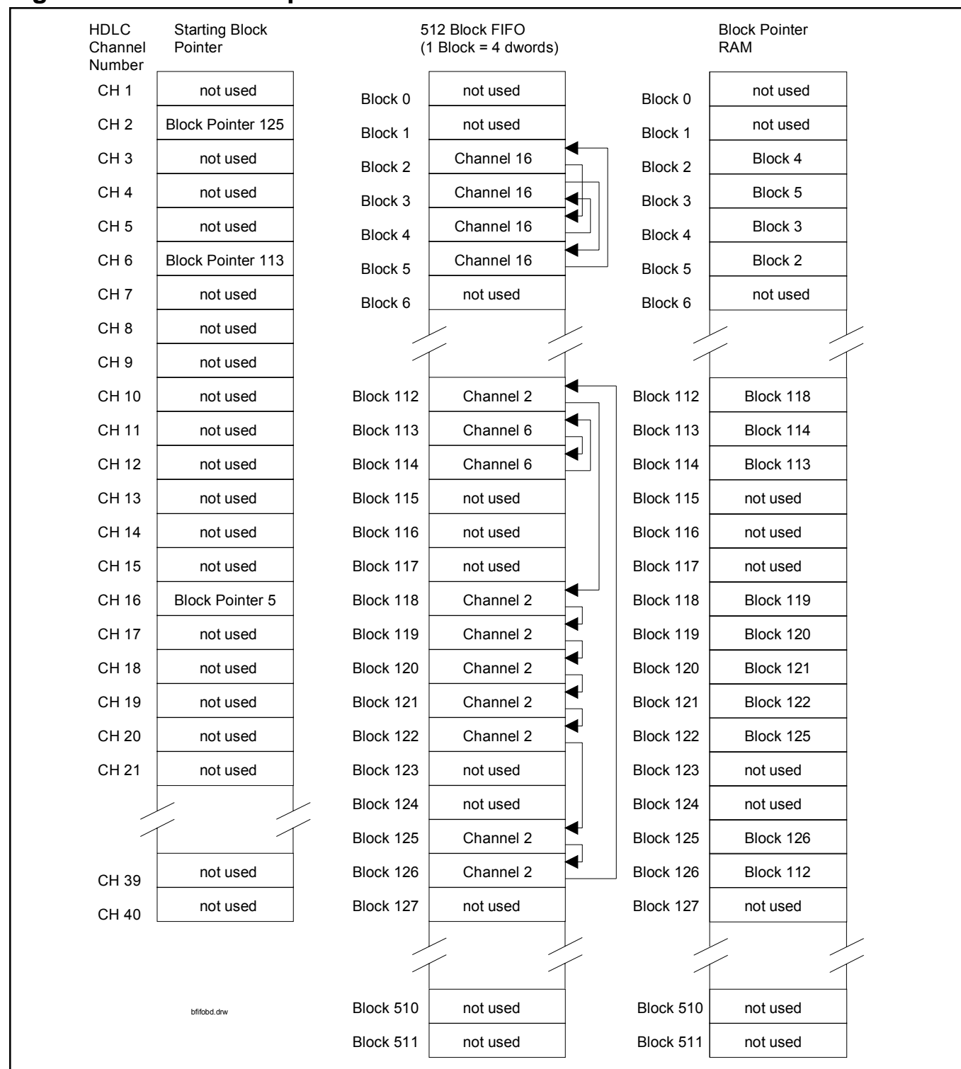
Figure 8-1. FIFO Example
