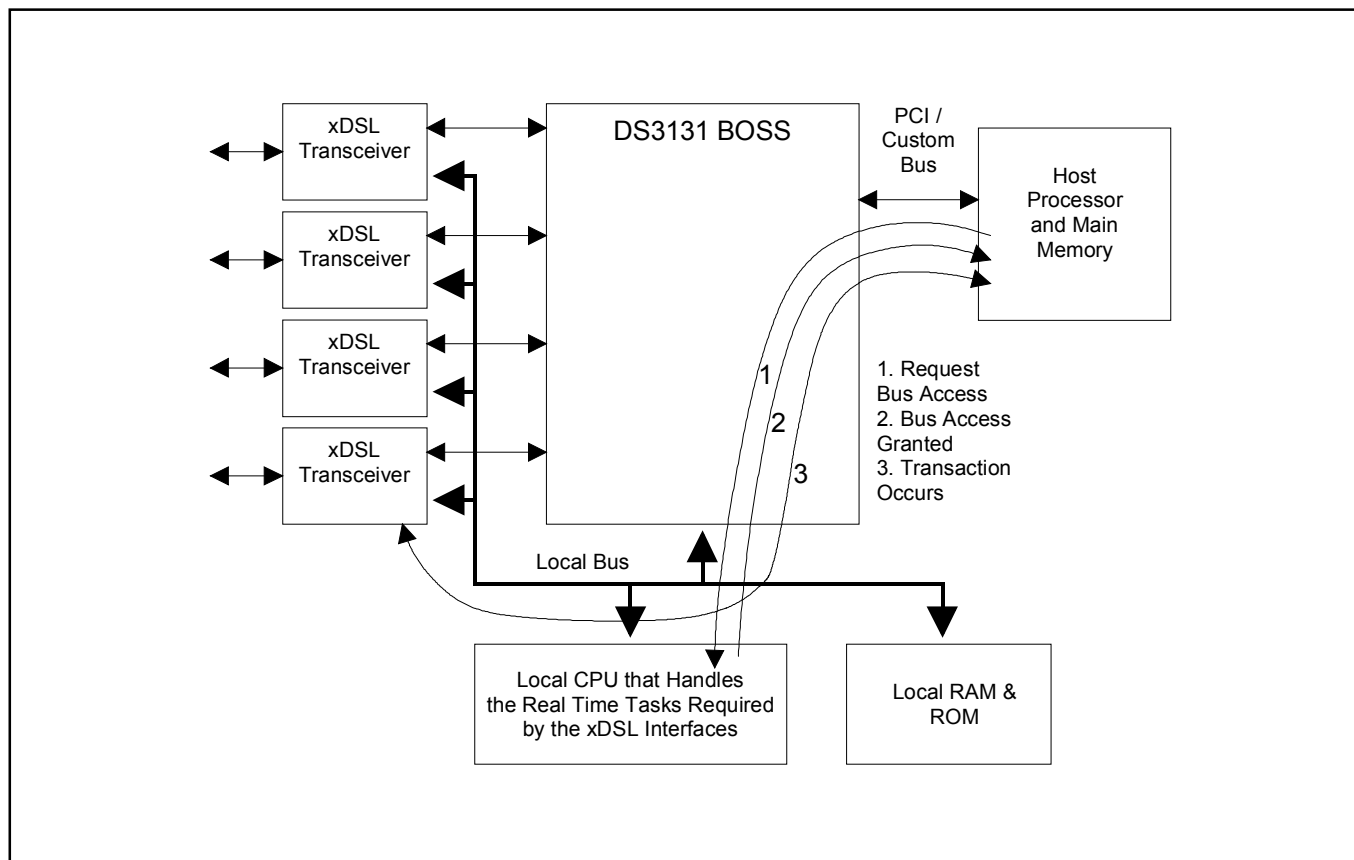
Figure 11-2. Bridge Mode with Arbitration Enabled
