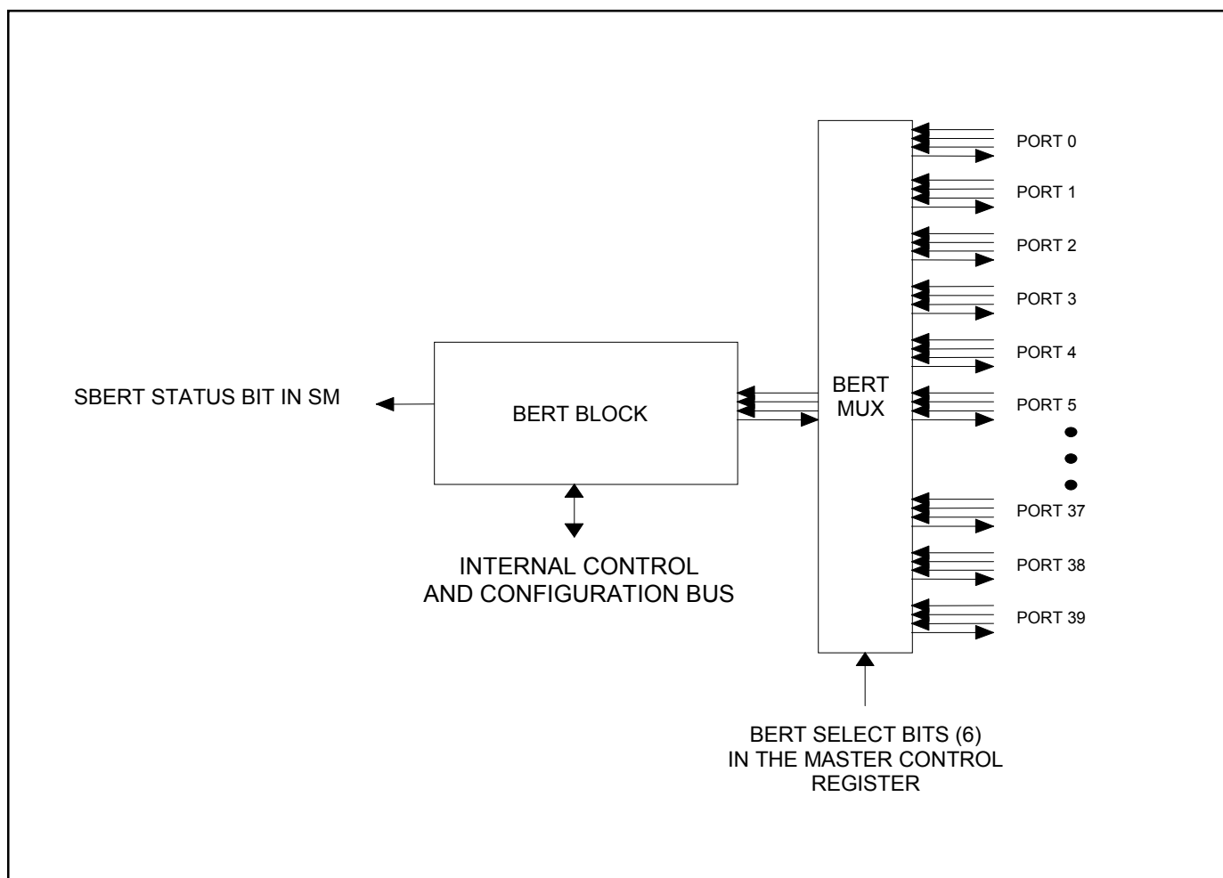
Figure 6-2. BERT Mux Diagram
