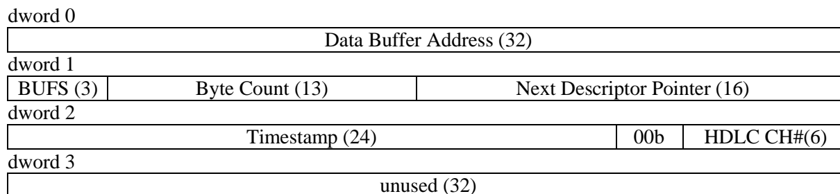
Figure 9-4. Receive Packet Descriptors
