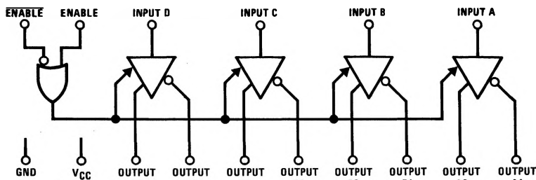
Dual-In-Line Package
