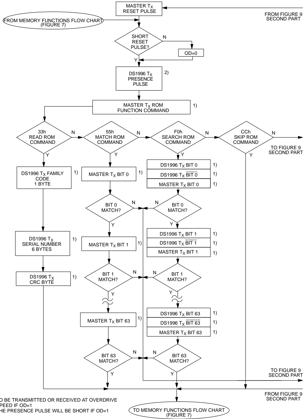
ROM FUNCTIONS FLOW CHART Figure 9
