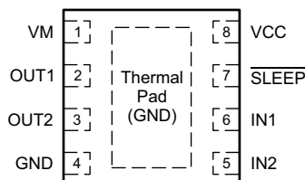
DRV8837 DSG Package (Top View)
