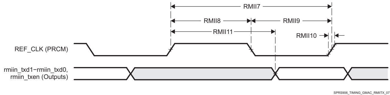
Figure 7-58. GMAC Transmit Interface Timing RMIIn Operation
