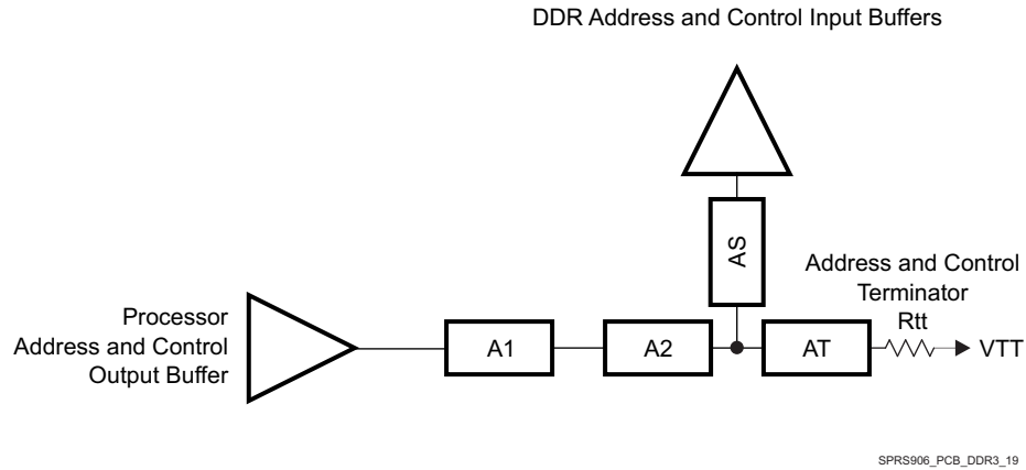
Figure 8-58. ADDR_CTRL Topology for One DDR3 Device
