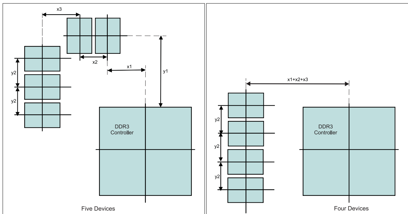
Figure 8-43. Placement Specifications
