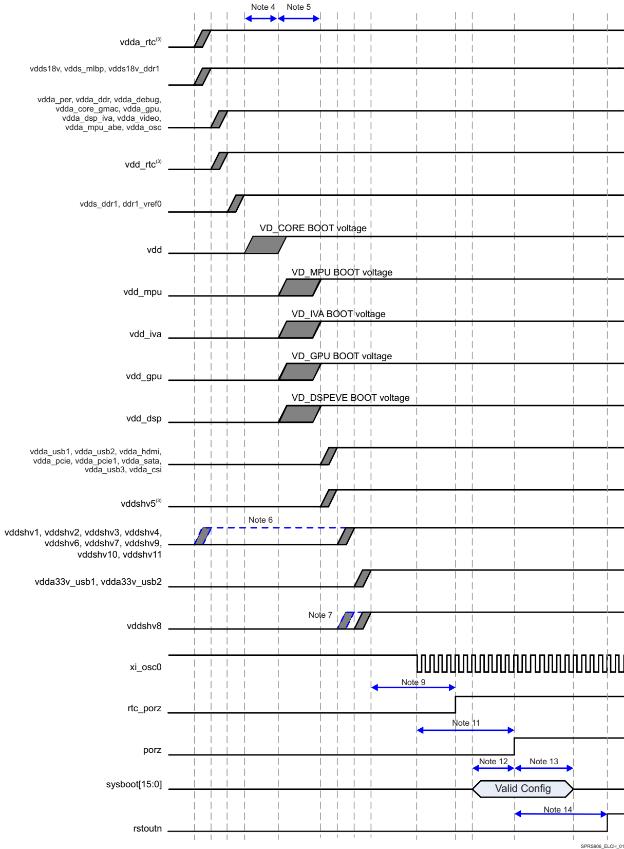
Figure 5-2. Power-Up Sequencing
