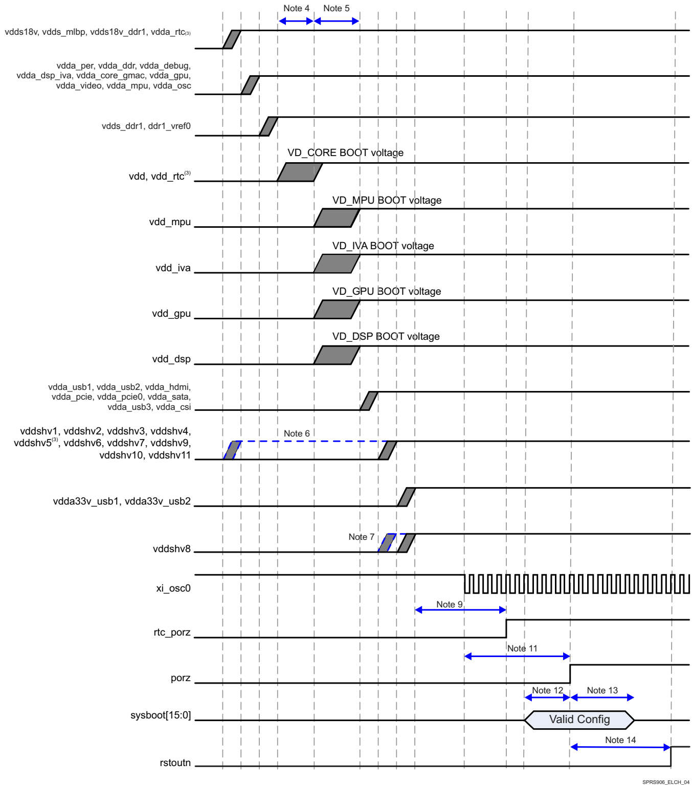
Figure 5-5. Power-Up Sequencing
