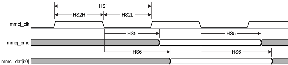
Figure 7-86. MMC/SD/SDIOj in - High Speed 3.3V Signaling - Transmitter Mode
