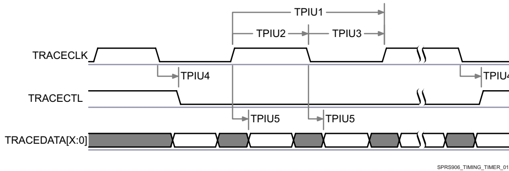
Figure 7-96. TPIU-PLL DDR Transmit Mode (1)
