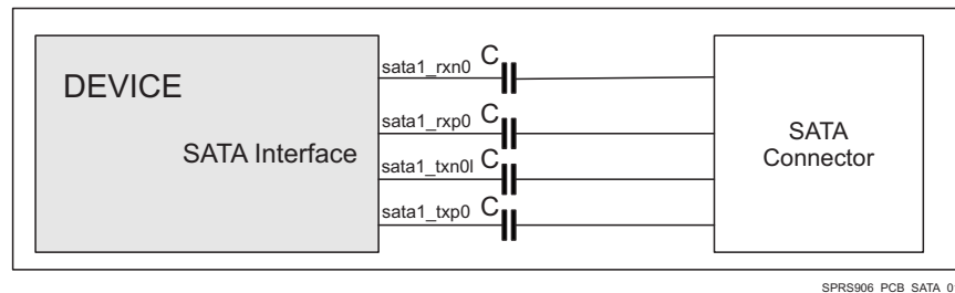
Figure 8-36. SATA Interface High Level Schematic
