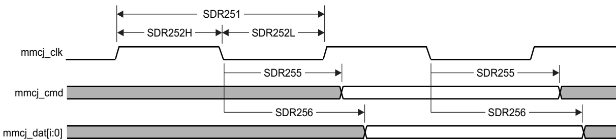
Figure 7-90. MMC/SD/SDIOj in - SDR25 - Transmitter Mode
