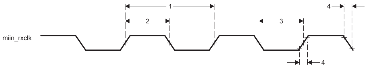
Figure 7-52. Clock Timing (GMAC Receive) - MII operation
