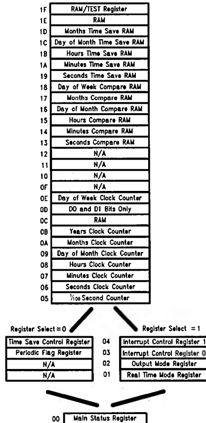
FIGURE 2. DP8573A Internal Memory Map
