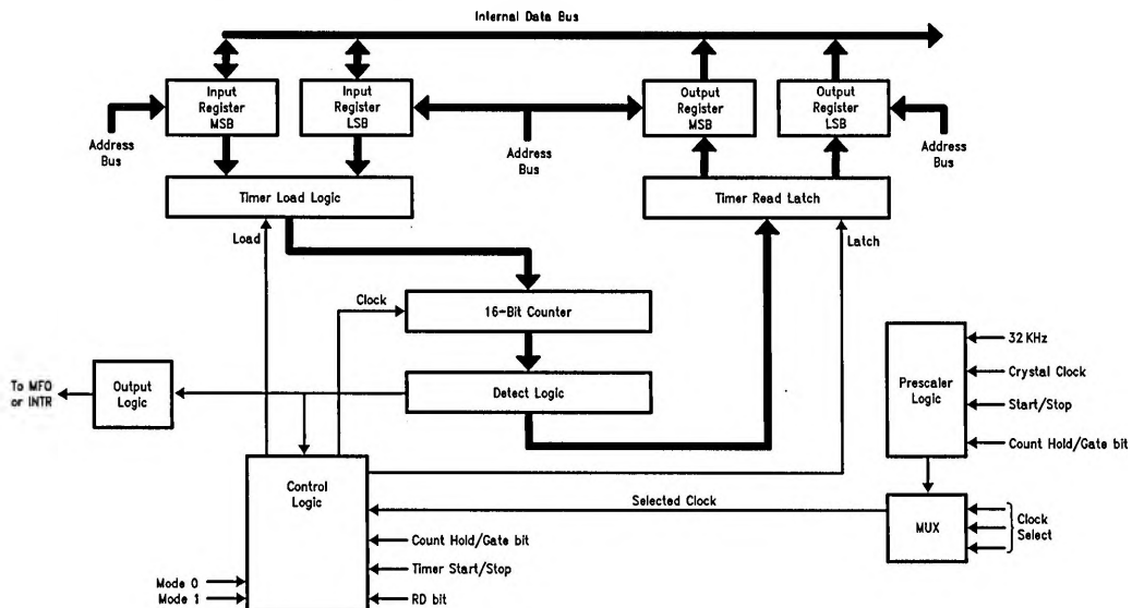
FIGURE 7. DP8571A Timer Block Diagram
