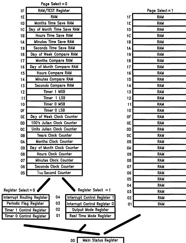
FIGURE 2. DP8571A Internal Memory Map
