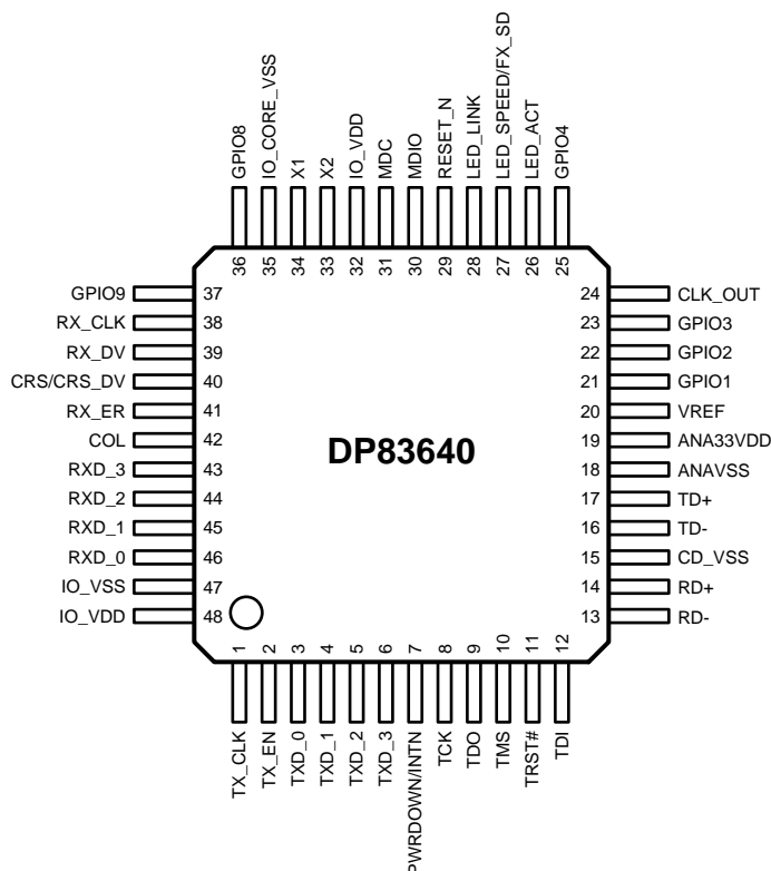
Figure 2-4. Top View
