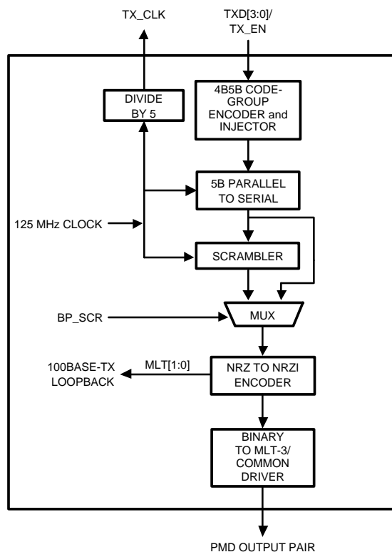
Figure 3-5. 100BASE-TX Transmit Block Diagram
