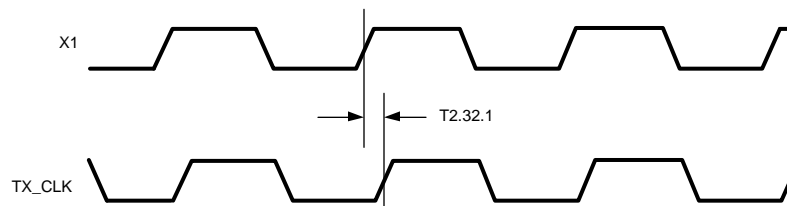
Figure 4-32. 100 Mb/s X1 to TX_CLK Timing
