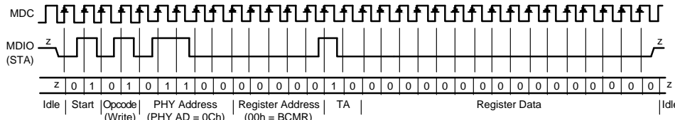
Figure 3-4. Typical MDC/MDIO Write Operation
