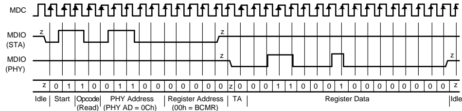
Figure 3-3. Typical MDC/MDIO Read Operation
