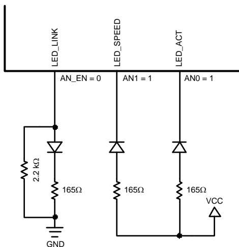
Figure 3-2. AN Strapping and LED Loading Example
