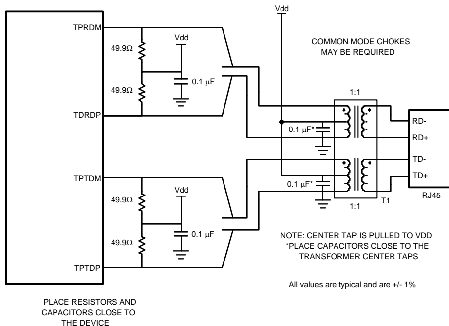
Figure 3-8. 10/100 Mb/s Twisted Pair Interface
