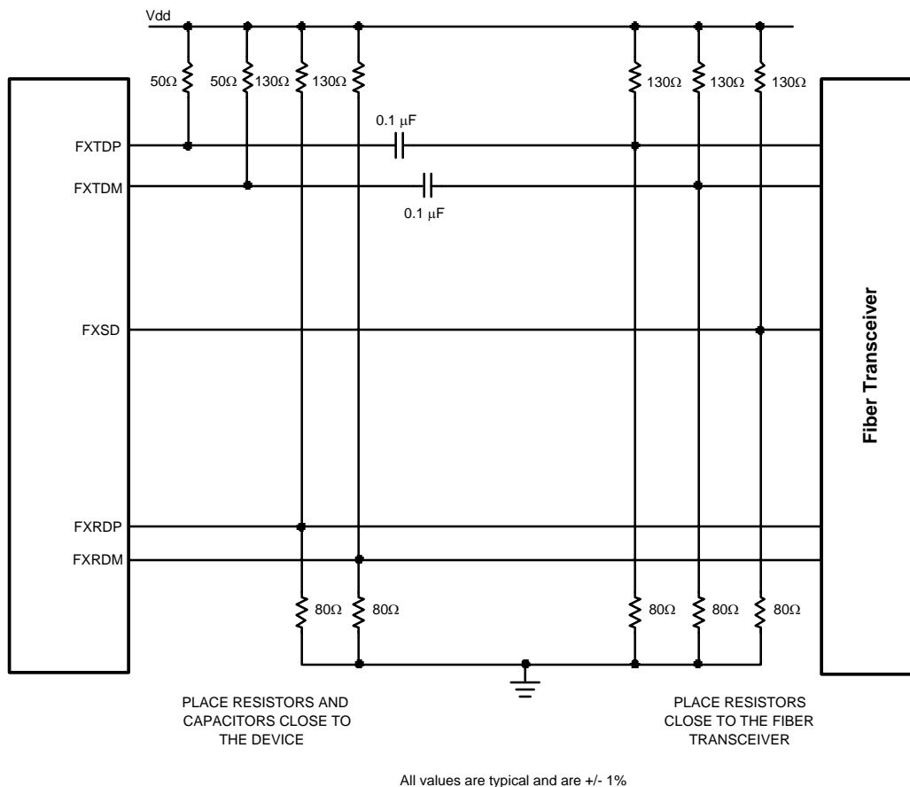
Figure 3-9. 100 Mb/s Fiber Pair Interface
