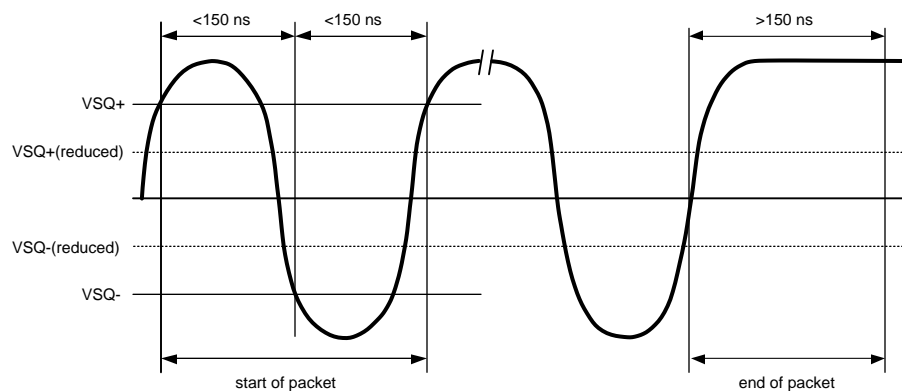
Figure 3-7. 10BASE-T Twisted Pair Smart Squelch Operation
