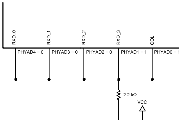
Figure 3-1. PHYAD Strapping Example
