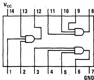
DM5411/DM7411
