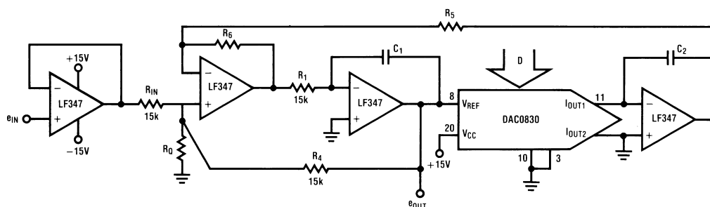
Figure 32. Variable f_0 , Variable Q_0 , Constant BW Bandpass Filter
