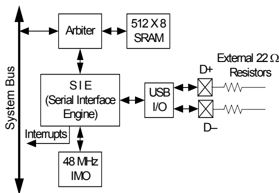
Figure 7-16. USB
