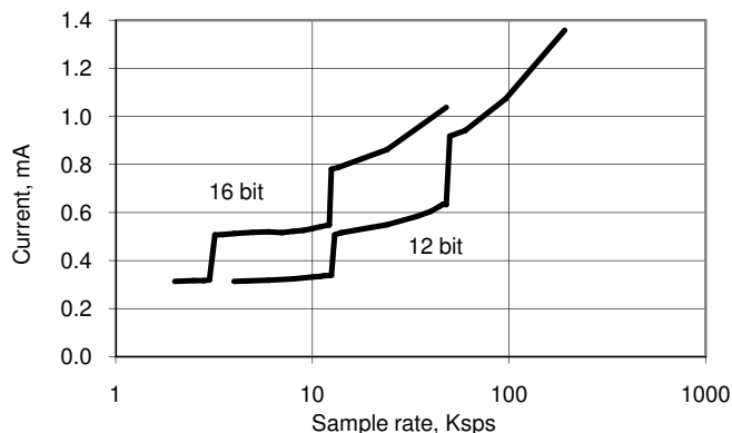
Figure 11-27. Delta-sigma ADC IDD vs sps, Range = \pm 1.024 V, Continuous Sample Mode, Input Buffer Bypassed
