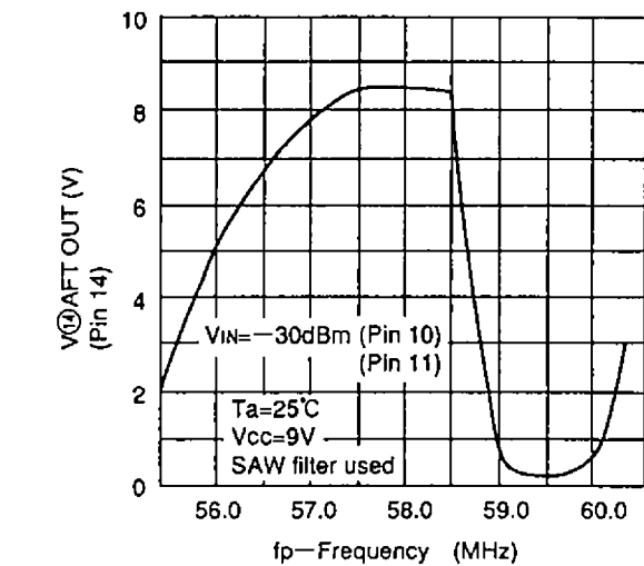
Pin 14 voltage vs. Frequency
