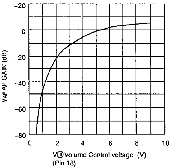
Audio amplifier gain vs. Pin 18 voltage
