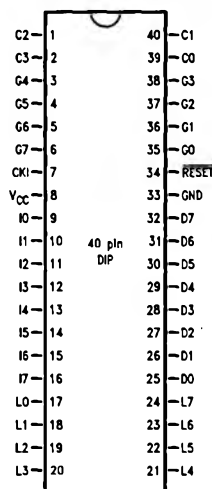
Dual-In-Line Package
