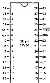
Dual-In-Line Package
