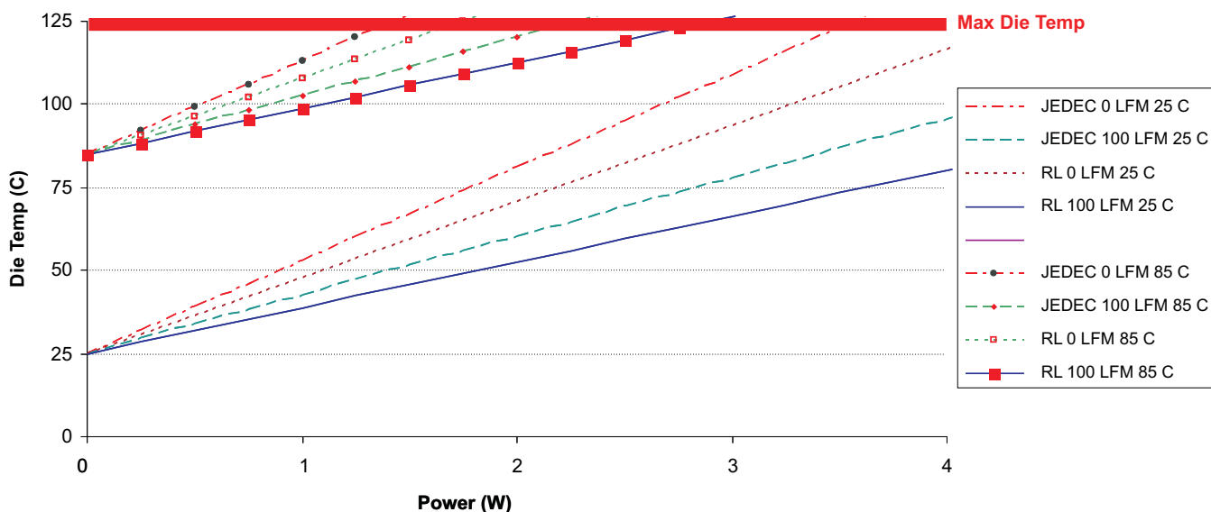
Figure 33. Die Temperature
